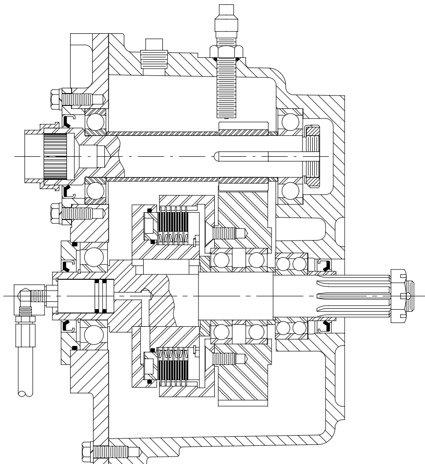
CROSS SECTION VIEW MODEL CM/CS MOUNTED HEAVY DUTY KC TRANSMISSION
