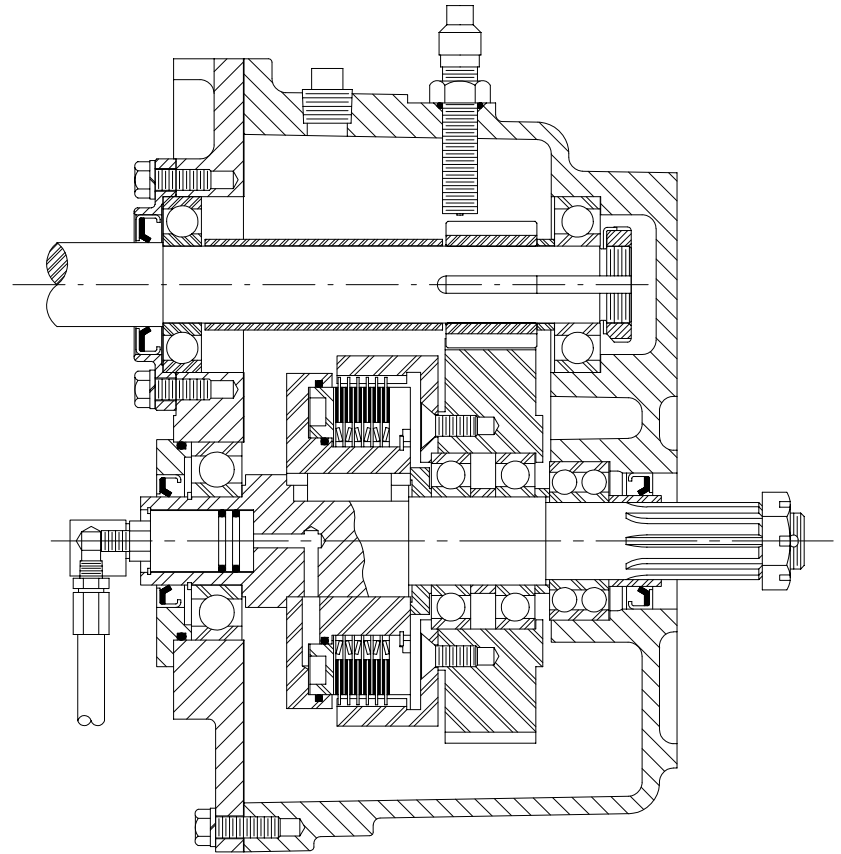
CROSS SECTION VIEW MODEL CL/CG, CLS/CGG MOUNTED HEAVY DUTY KC TRANSMISSION
