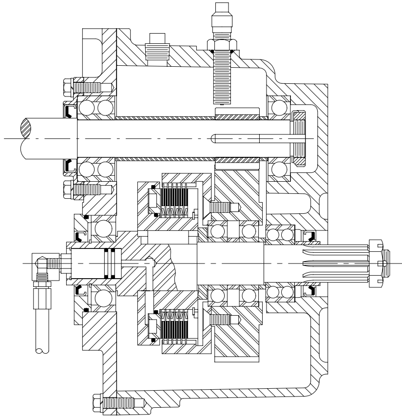
CROSS SECTION VIEW MODEL CX MOUNTED HEAVY DUTY KC TRANSMISSION
